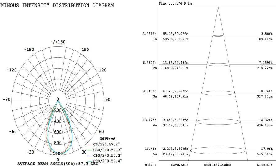
LUMINOUS INTENSITY DISTRIBUTION DIAGRAM
